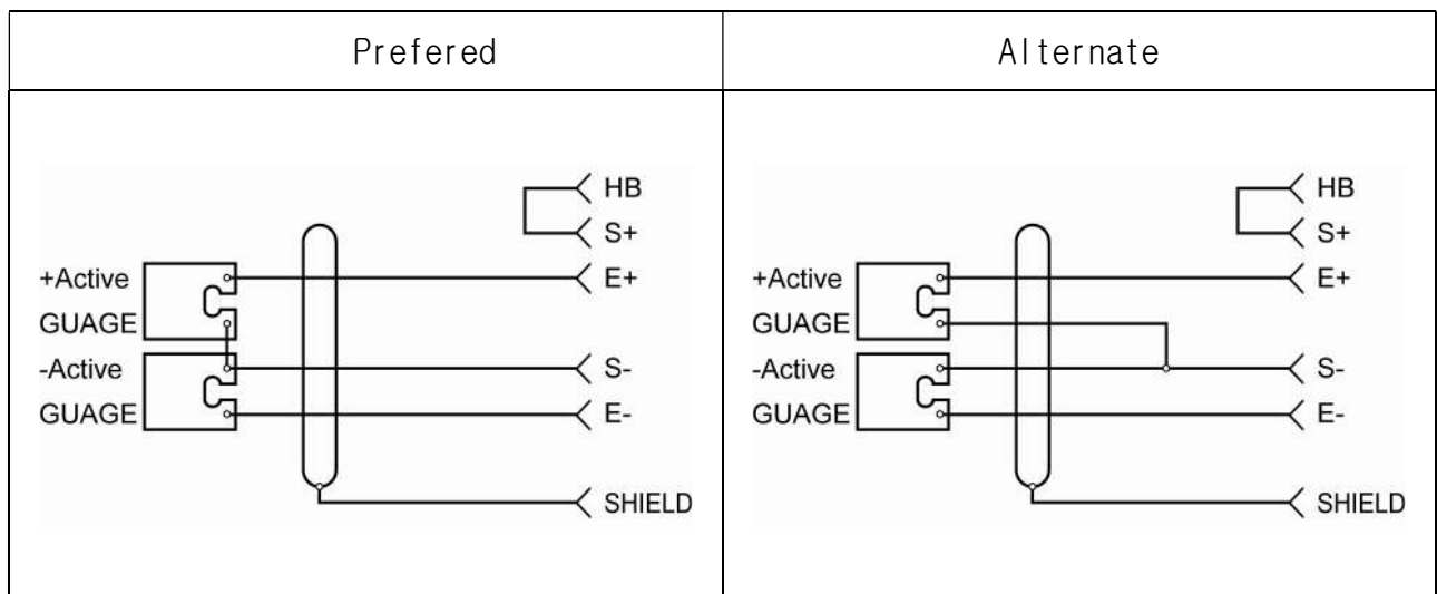
Half Bridge 결선
