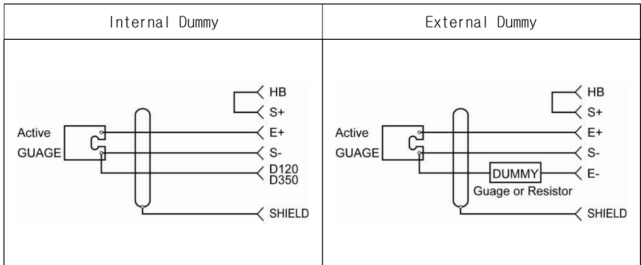
Quarter Bridge 결선
